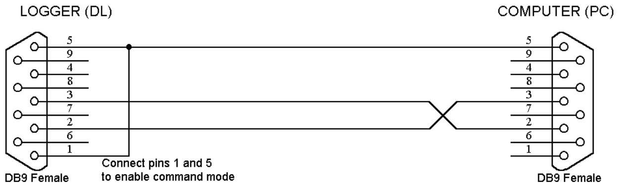
Download Cable Circuit
